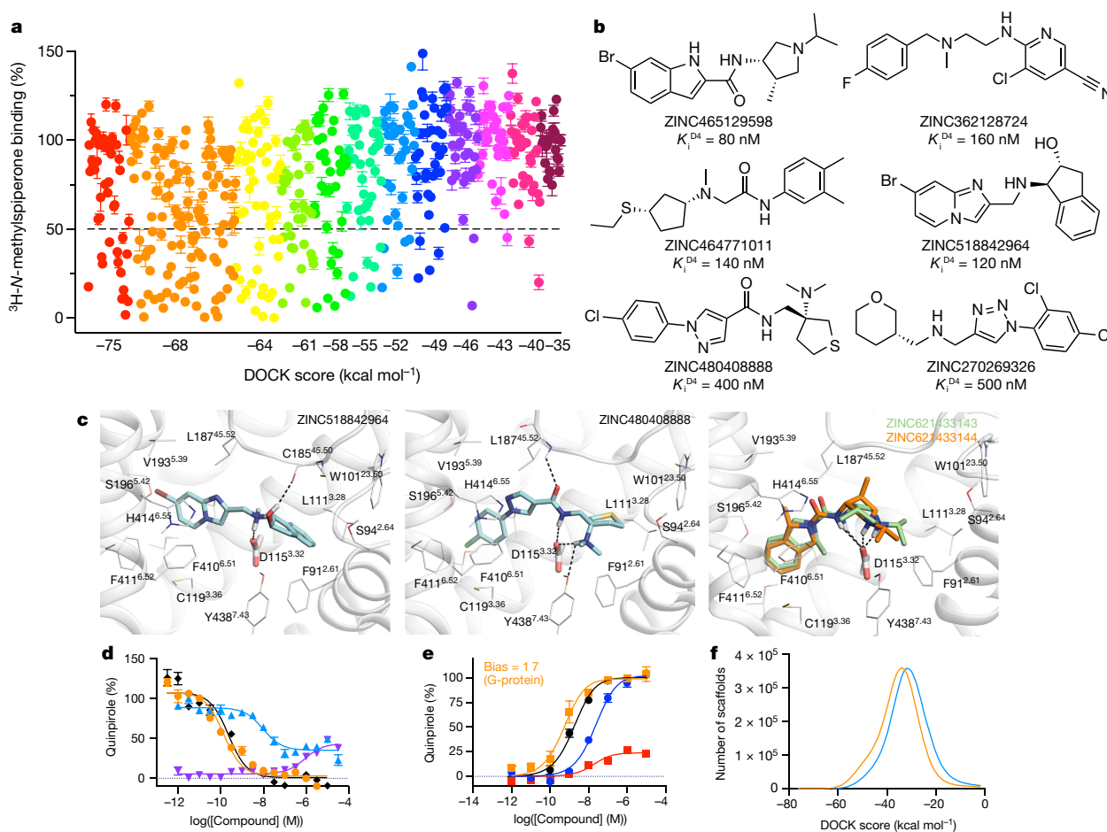
Fig. 3 | Testing 549 molecules at different docking ranks against the D_4 receptor. a , Displacement of the antagonist ^3H - N -methylsiperone by each of the 549 molecules tested at 10 \mu\text{M} . Data are mean \pm s.e.m. of three assays. The molecules are coloured by their docking score. The number of molecules with substantial activity ( <50\% remaining radioligand, below the dashed line) diminishes with docking score. b , Six active compounds, each with a different scaffold. c , Docked poses of ZINC518842964 (left), ZINC480408888 (middle) and superposed 21433143 and 621433144 (right). The receptor helices are shown as ribbons, the conserved D115 3.32 is shown as sticks, interacting residues within 4 Å of the docked molecules are shown as lines. Ballesteros–Weinstein residue numbers are shown as superscripts. Modelled hydrogen bonds are shown as dashed
