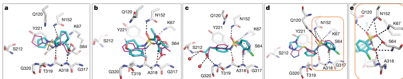
Fig. 2 | Structural fidelity between docked-predicted and crystallographically determined poses of the new \beta -lactamase inhibitors. Crystal structures of the inhibitors (carbons in cyan) overlaid with their docking predictions (magenta). AmpC carbon atoms are shown in grey, oxygens in red, nitrogens in blue, sulfurs in yellow, chlorides in green and fluorides in light blue. Hydrogen bonds are shown as black dashed lines. a–d , AmpC in complex with ZINC547933290 ( a ; Protein Data Bank (PDB) 6DPZ, r.m.s.d. = 1.3 Å) and 275579920 ( b ; PDB 6DPY, r.m.s.d. = 1.2 Å for the warhead), the 1.3 \mu M inhibitor 339204163 (PDB 6DPX; r.m.s.d. = 0.98 Å) and its 77 nM analogue 549719643 ( d ; PDB 6DPT, r.m.s.d. = 1.52 Å). e , Close-up of the 549719643 phenolate in the oxyanion hole. Extended Data Fig. 4 shows the electron densities.
