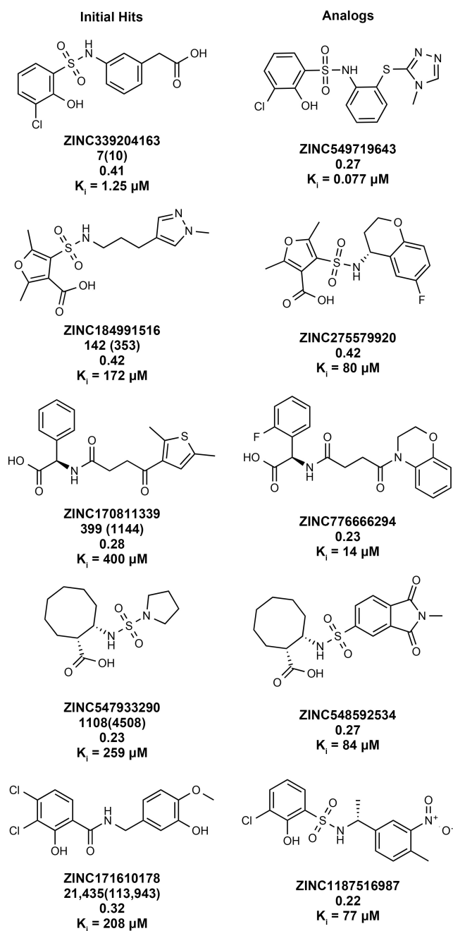
Extended Data Fig. 2 | Initial hits and selected analogues against AmpC. The five initial hits are shown in the left column. Under each compound, the first row includes the ZINC identifier; the second row is the cluster rank (position in cluster head list sorted by DOCK score) with global rank (position in unclustered hit list sorted by DOCK score) shown in brackets; the third row is the Tc value (Tanimoto coefficient to known AmpC inhibitors in ChEMBL); the fourth row is the K_i value. Five selected analogues for the corresponding hits are shown in the right column. Under each compound, the first row includes the ZINC identifier; the second row is the Tc value; and the third row is the K_i value.
