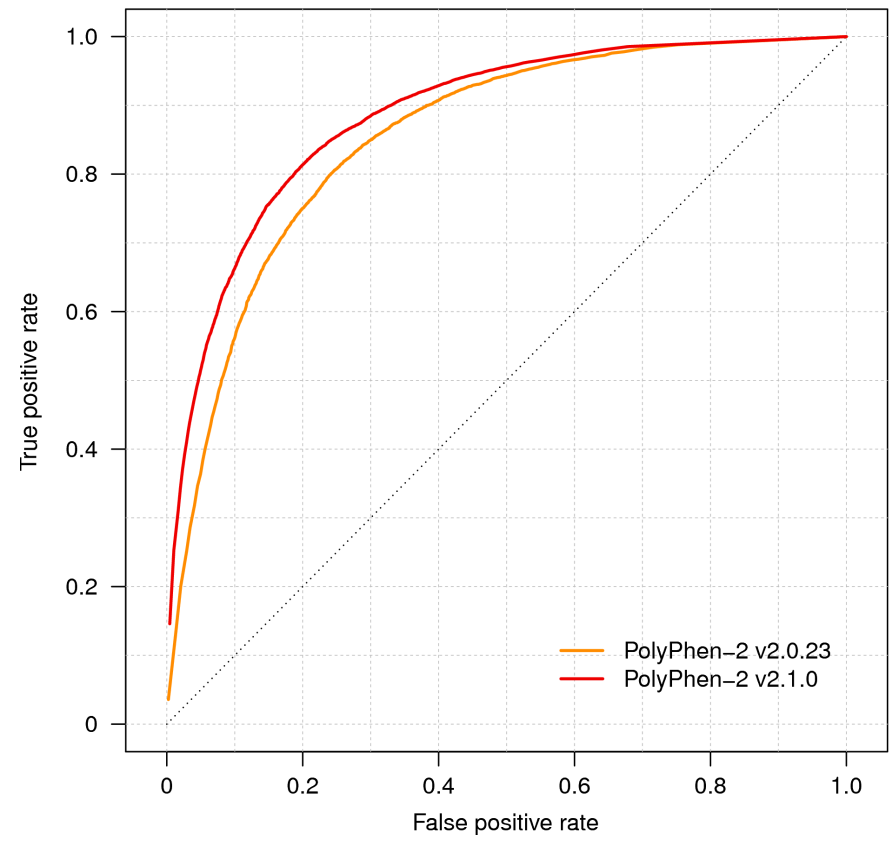
HumVar / UniRef100
